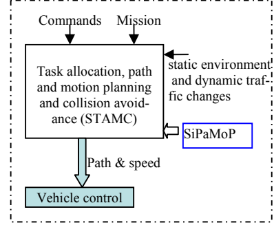
Fig. 2. STAMC approach
