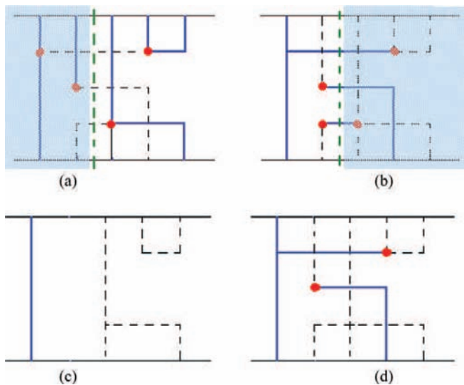
Fig. 6. Crossover operation
