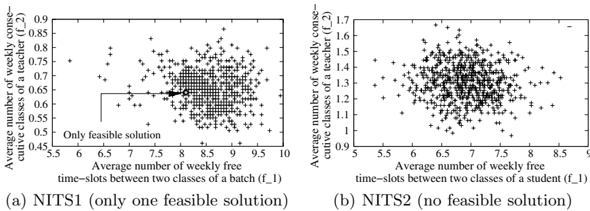
Fig. 6. NITS1 and NITS2 with relaxed student/batch and teacher-clash constraints ( p_c = 0.90 , p_m = 0.01 and r_s = 0.125 ).
