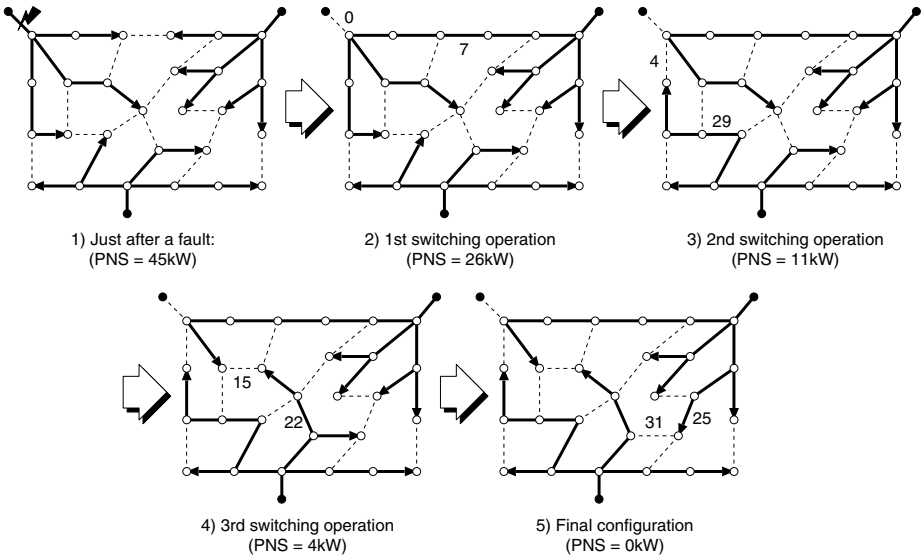
Fig. 12. Optimal sequence of switching operations (CASE-2)
