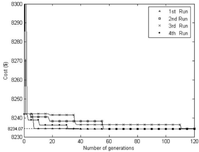
Fig. 10. Convergence characteristics of the proposed method with different initial conditions in case B
