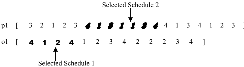
Fig. 7. Exchange of partial schedules
