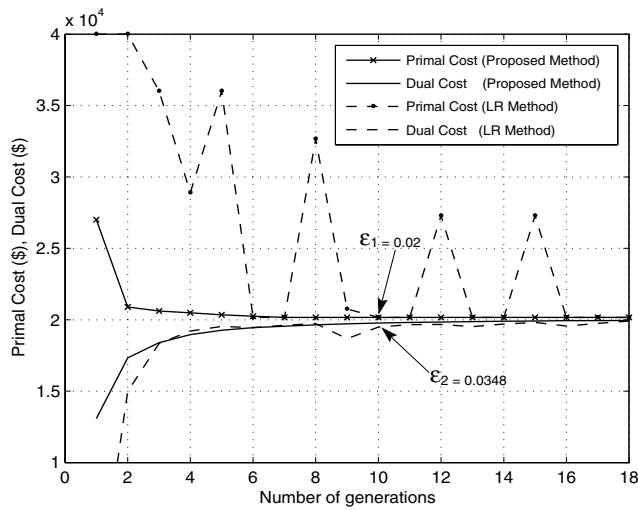
Fig. 5. Comparison of convergence curves between the proposed method and the LR method ( \epsilon_1 - Duality gap of the proposed method and \epsilon_2 - Duality gap of the LR method)
