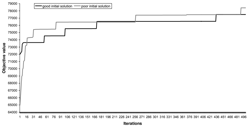
Fig. 3. Performance of hyperheuristic TabuEventAdaptive(80) on Dataset2 starting from different initial solutions.
