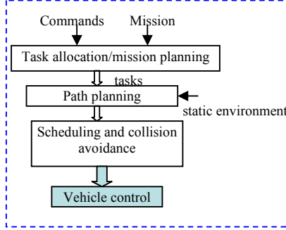
Fig. 1. Traditional sequential approach
