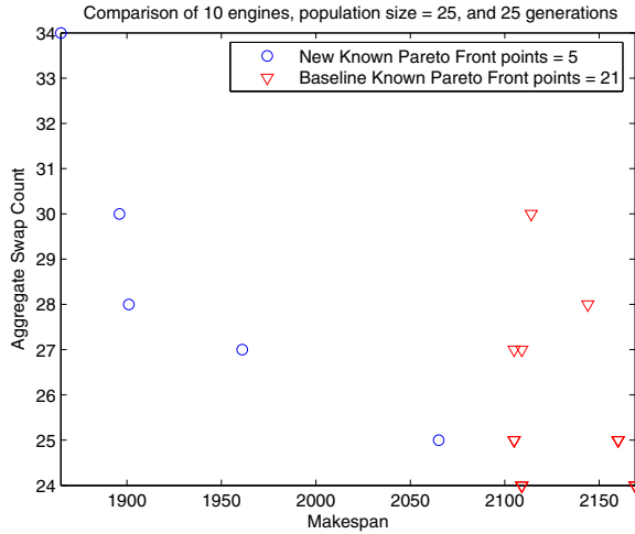
Fig. 37. Comparison of the Pareto front members for the 10 engine instance.
