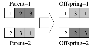
Fig. 1. Traditional 1-point crossover.
