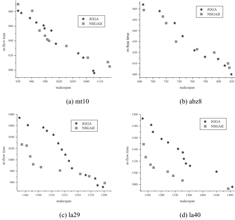
Fig. 14. Final Pareto-optimal front
