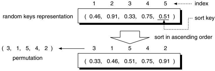
Fig. 6. A simple example of random keys representation
