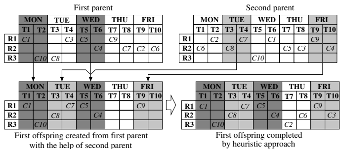
Fig. 2. Generation of the first offspring using XVRA.
