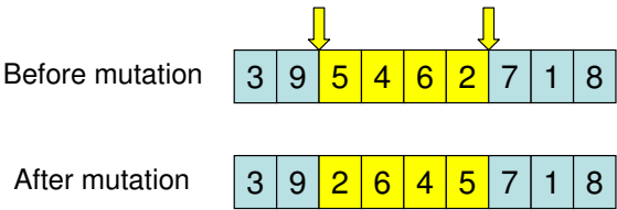
Fig. 27. Example of inversion mutation for a 9-job, job-based chromosome.
