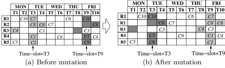
Fig. 3. Mutation for Reshuffling Resource Allocation (MRRRA).
