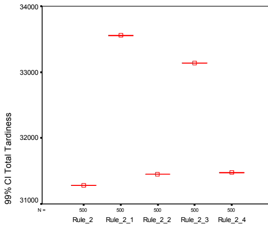
Fig. 8. Mean total tardiness with 99% confidence interval of Rule_2 and its modified dispatching rules after 500 runs
