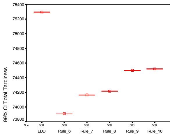
Fig. 7. Mean total tardiness with 99% confidence interval of EDD and Rule_6 to Rule_10 after 500 runs
