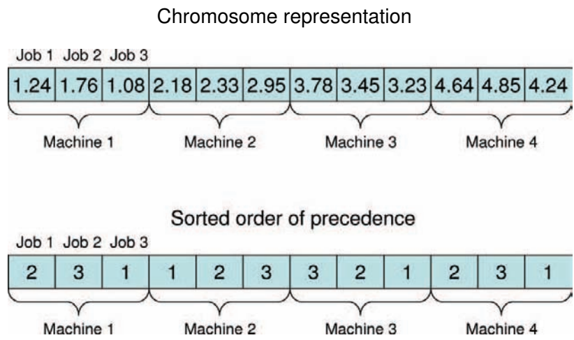
Fig. 12. Example of a random key chromosome representation for a three-job, four-operation job-shop.
