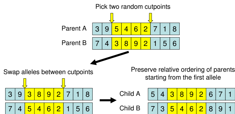
Fig. 19. Example of a variant of the order crossover operator. The relative ordering of the parent is referenced to the start of the chromosome.
