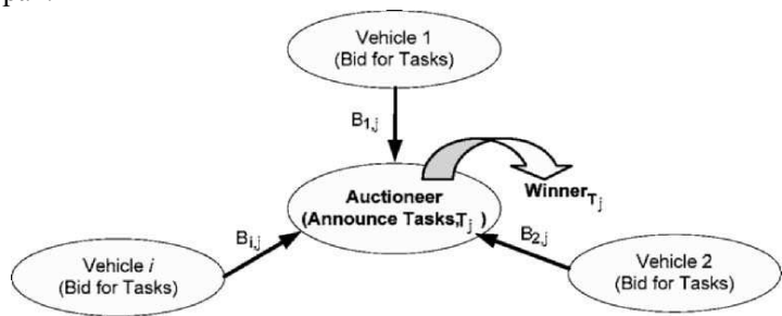
Fig. 11. Auction Process
