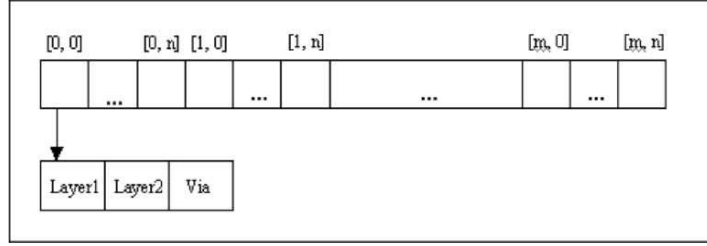
Fig. 3. Chromosome representation
