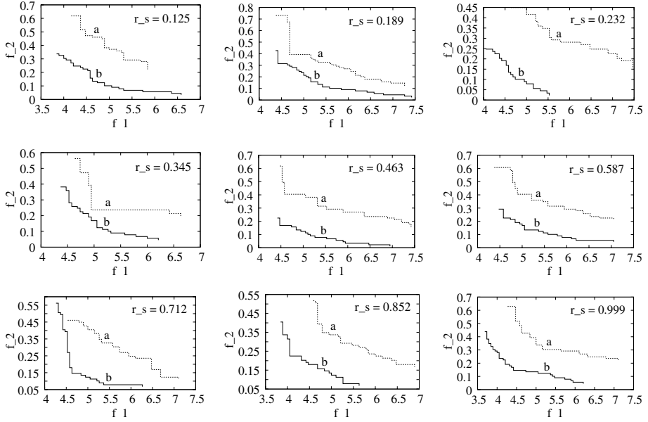
Fig. 10. Comparison of Pareto fronts of NITS1, obtained under different initial solutions ( r_s ) and evolving p_m . Curve (a): combined XVRA ( p_c=0.90 ) and MRRA, and curve (b): only MRRA.
