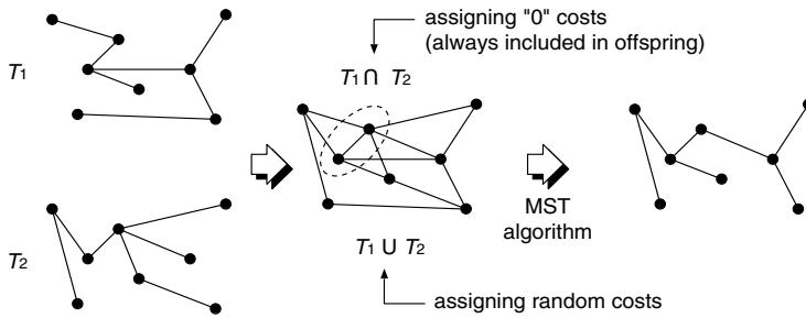
Fig. 4. Crossover operation in the first stage GA
